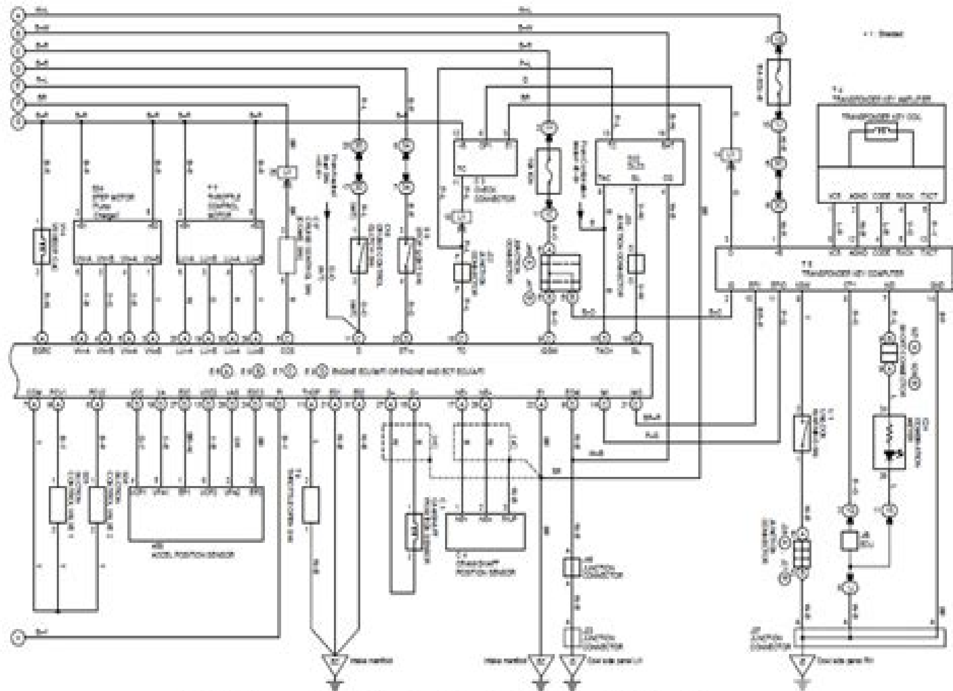
2000 Toyota Land Cruiser Prado Electrical Wiring Diagram
