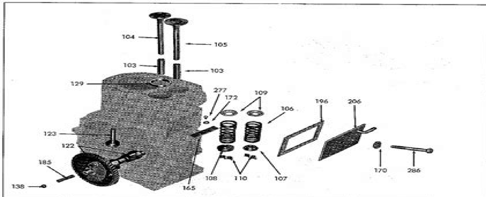
VALVES and CAMSHAFT GROUP
