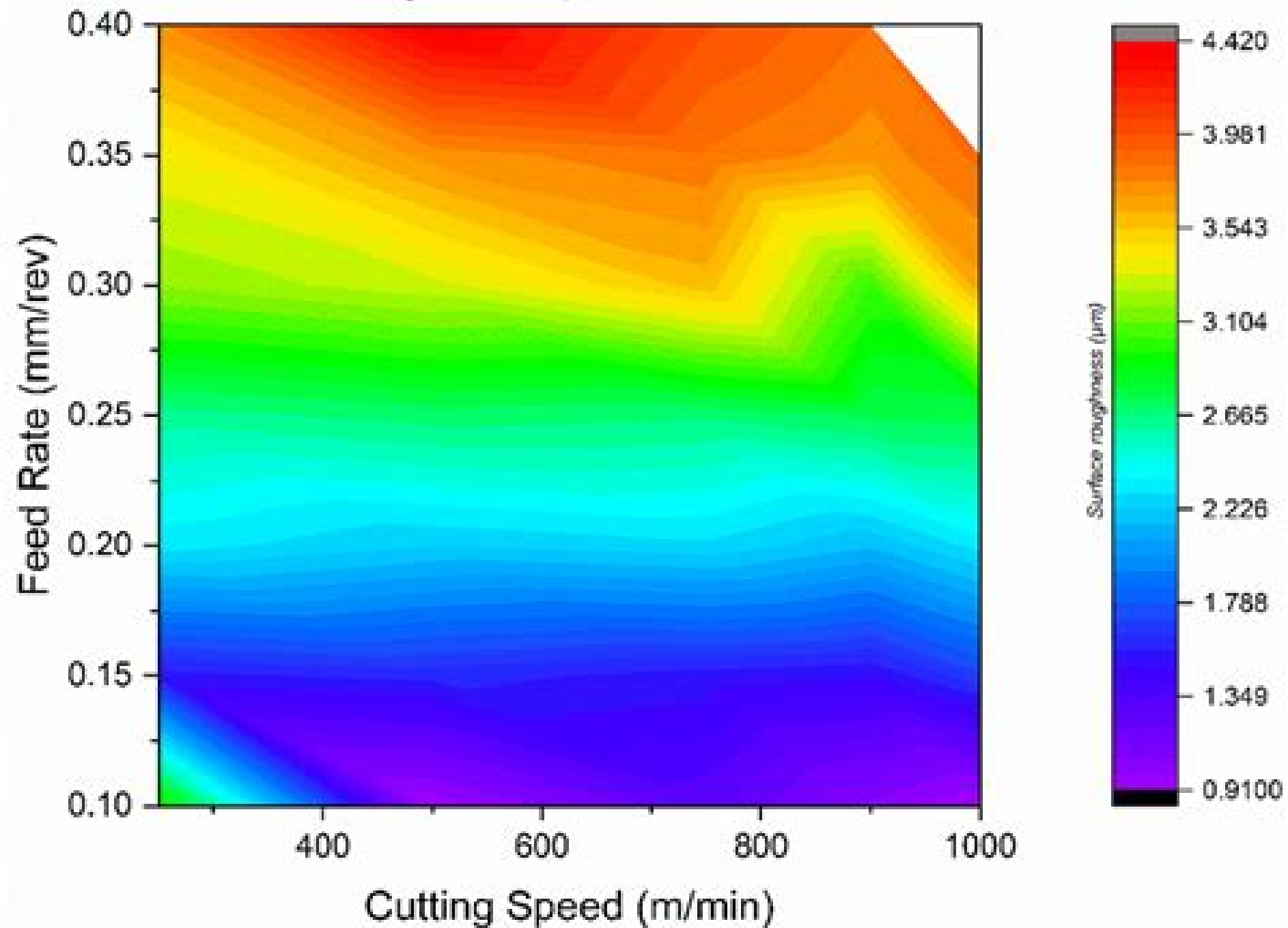
Surface roughness map for Aluminum 2014
