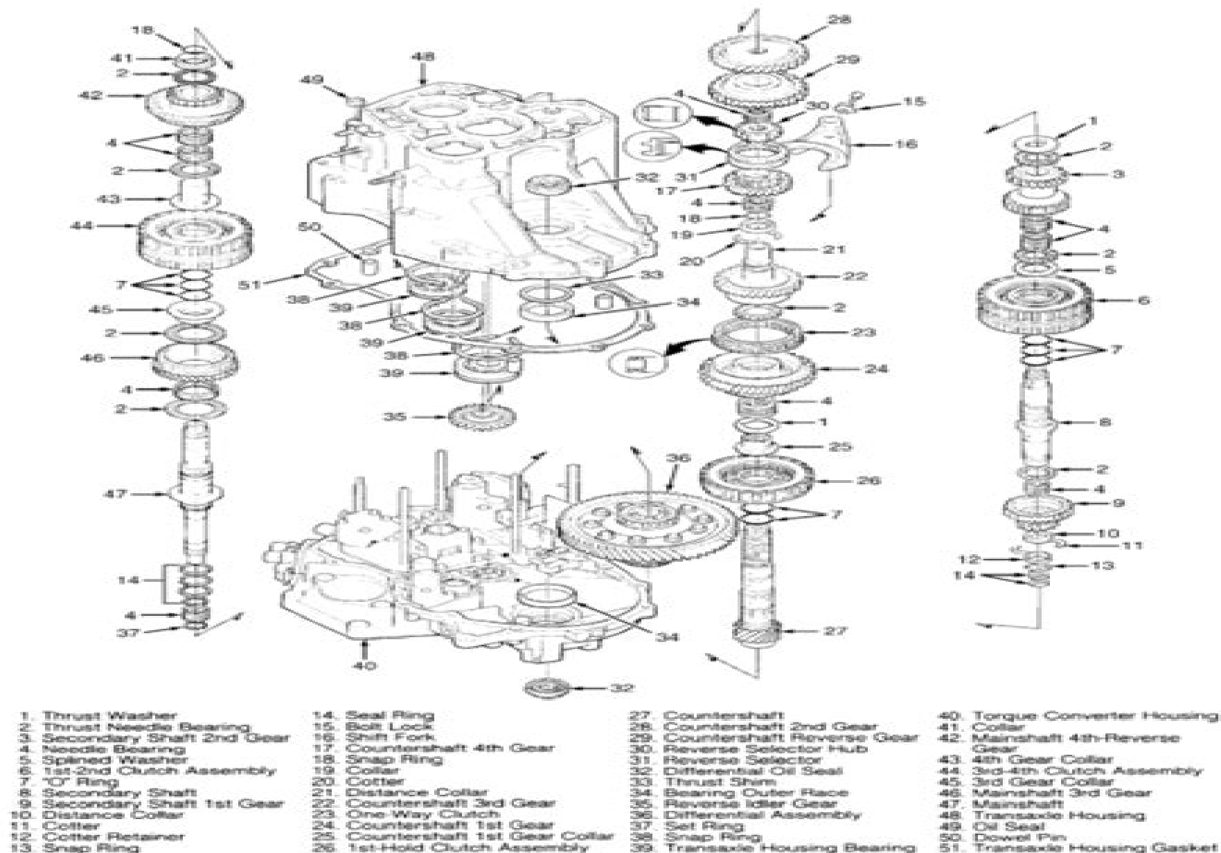
Fig 6: Exploded View Of Transaxle Housing & Components
