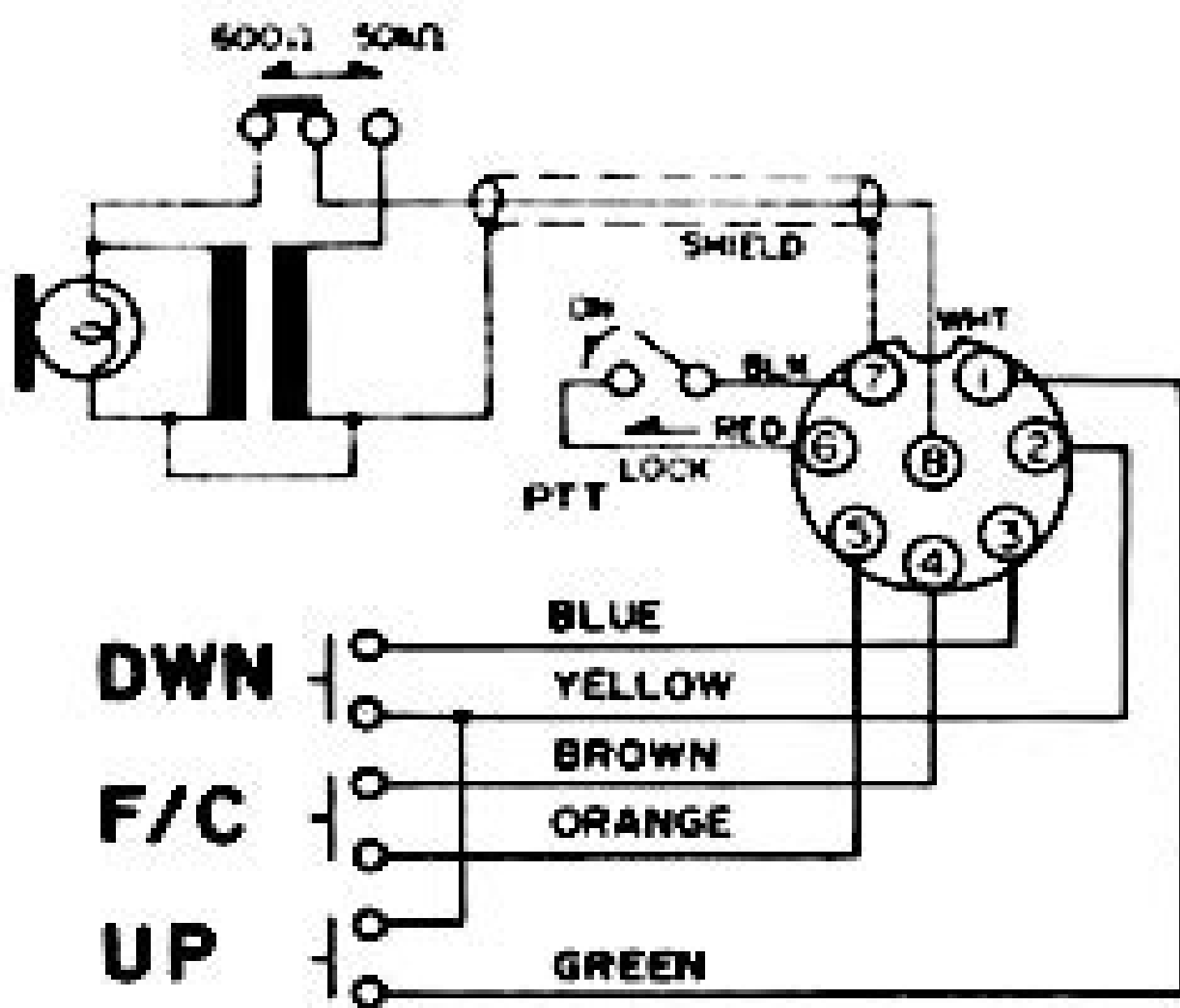
YM-38 MICROPHONE CONNECTIONS
