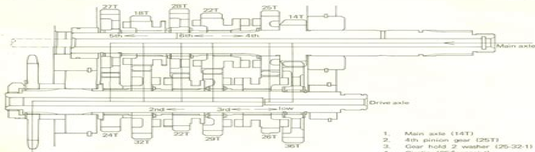
Sectional View of Transmission (6-Speed)
