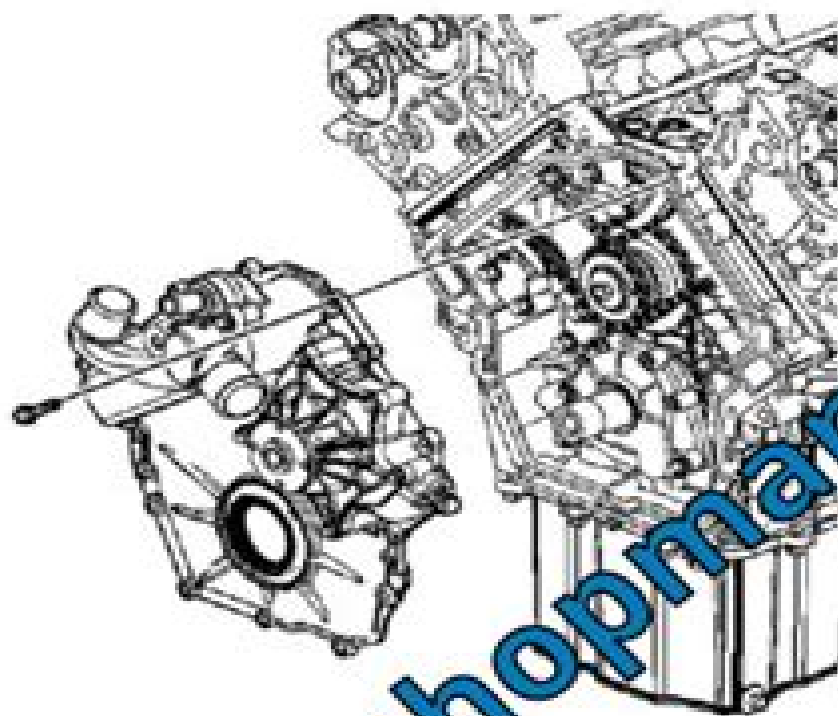
Fig. 49: View Of Engine Front Cover Assembly Components, Crankshaft Balancer. Courtesy of GENERAL MOTORS CORP.
