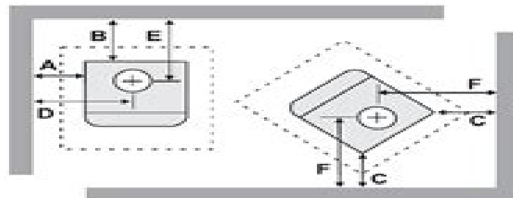
Residential Installation "C" Vent (Single Wall)
