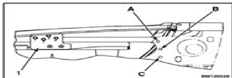
Figure 7. Gas Spring Installation, Lift Truck Models GLP/GDP16VX, GLP/GDP18VX, GLP/GDP20SVX (GP/GLP/GDP030VX, GP/GLP/GDP035VX, GP/GLP/GDP030SVX) (C810) and GLC20-35VX (GC/GLC040-070VX, GC/GLC055SVX) (A910)
