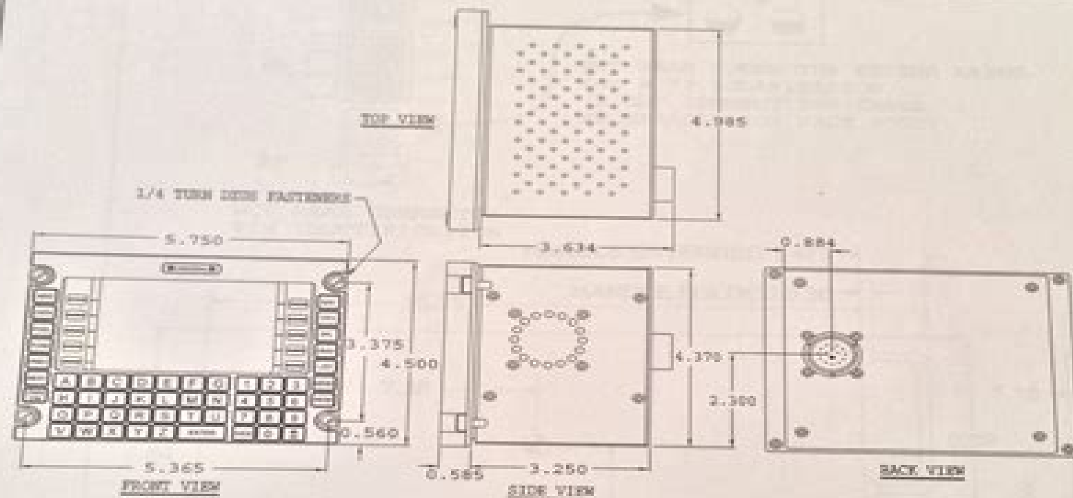
4" FPCDU Outline Drawing
