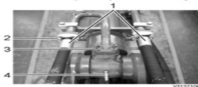
Figure 3752 Arm cylinder hydraulic hoses, removal
