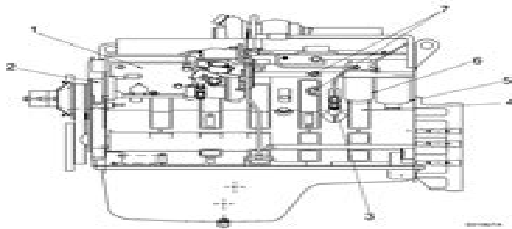
Figure 1 Engine, structure
