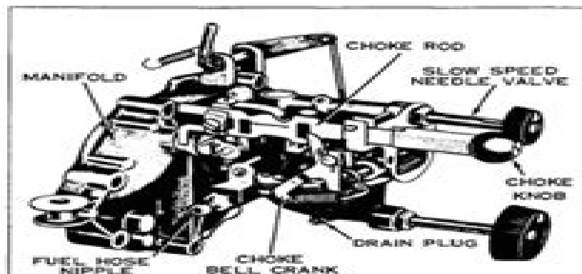
Figure 4-2. Carburetor for Late 12 H.P. Motors
