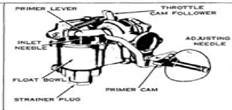
Figure 4-3. Carburetor for 3 H.P. Motors
