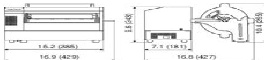
Dimensions in inches + (mm)
