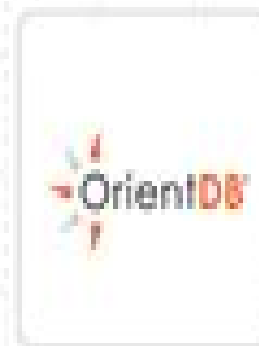
OrientDB
