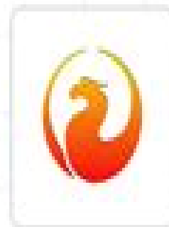
FirebirdSQL
