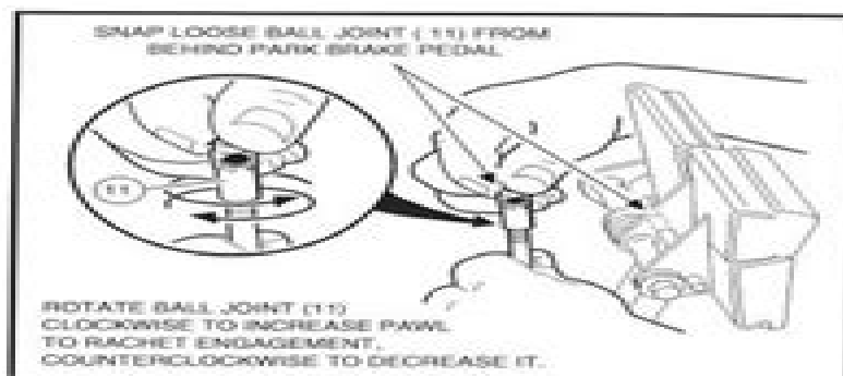
Figure 5-7 Brake Rod Adjustment
