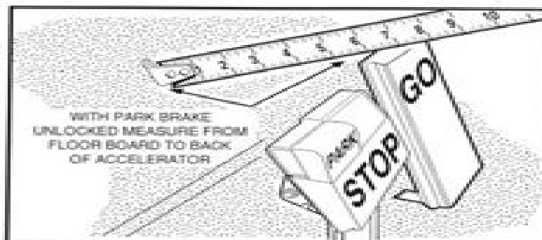
Figure 5-5 Measure Accelerator Pedal Height
