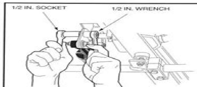
Figure 5-8 Accelerator Pedal Height Adjustment
