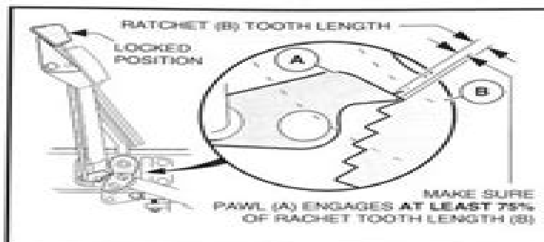
Figure 5-6 Ratchet/Pawl Tooth Engagement
