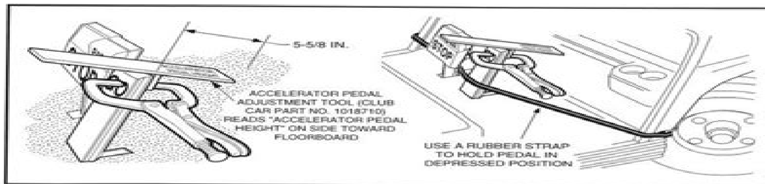
Figure 5-9 Accelerator Pedal Height Adjustment
