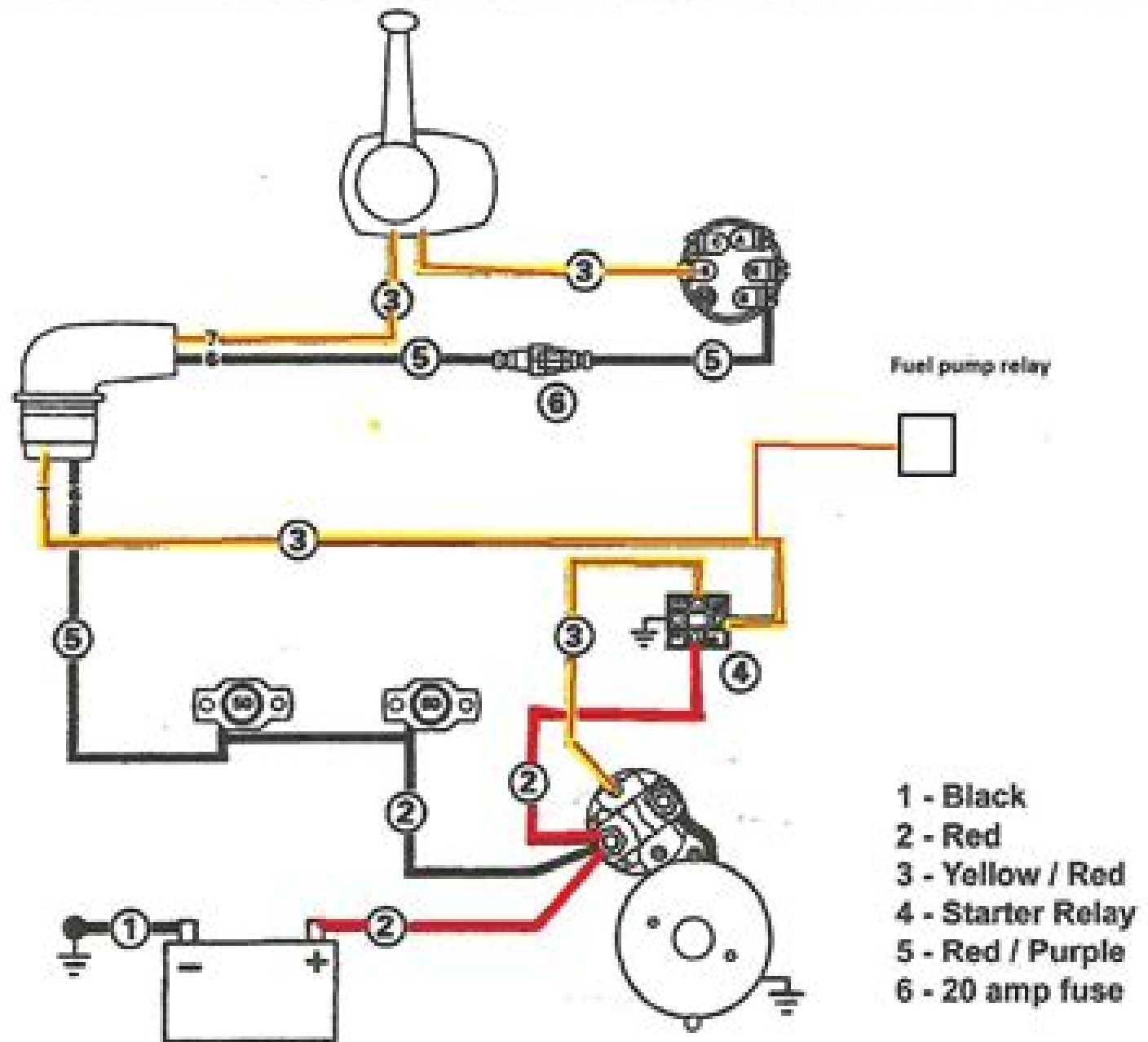
Fig. 160 Starting system wiring schematic—1996-98 3.0L, 4.3L and 5.7L engines (carburetor)
