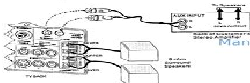
Amplifier and Dual Surround Speaker Connections
