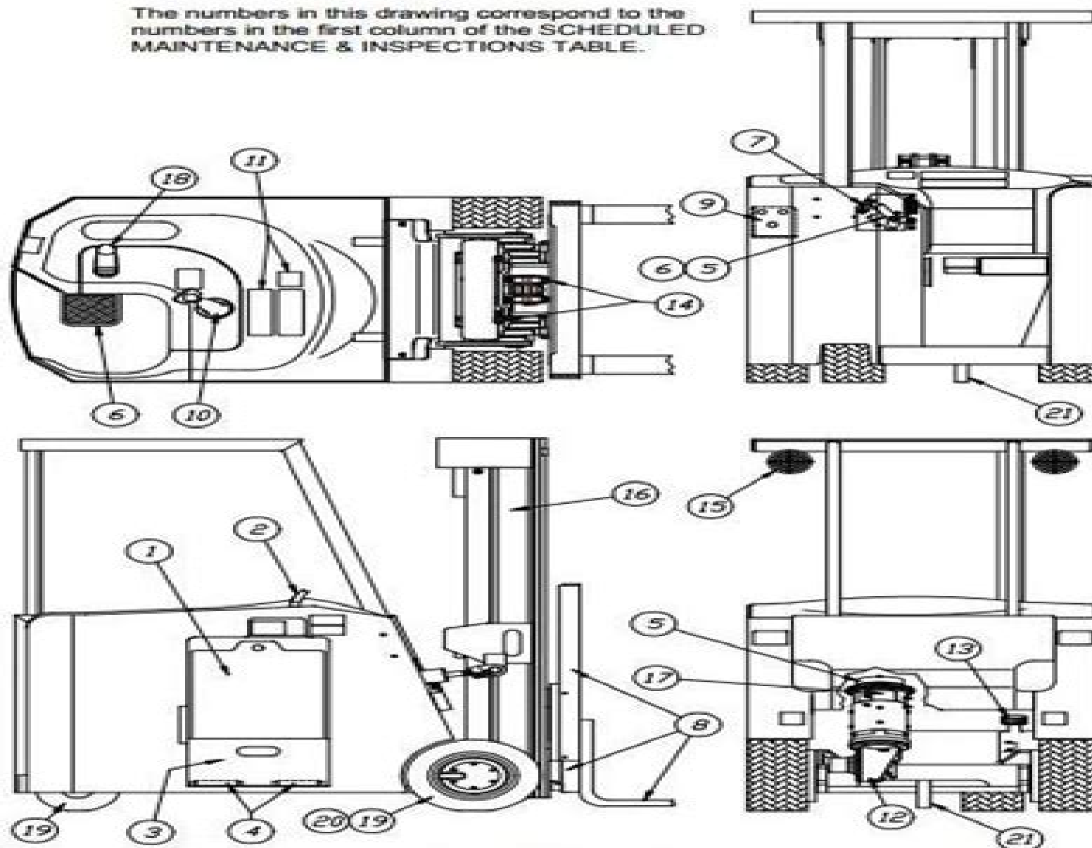
FIG. 10.1 - SCHEDULED MAINTENANCE AND INSPECTION POINTS
