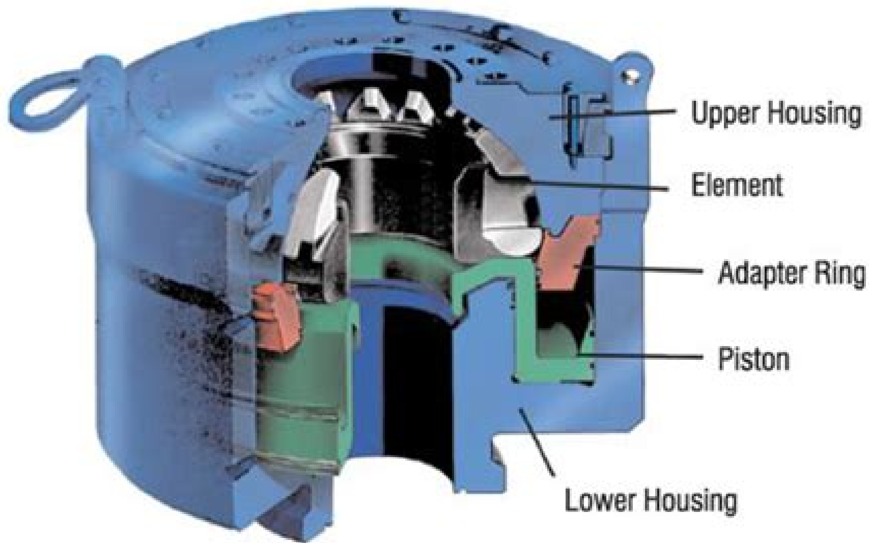
Figure 2-3. Shaffer® Wedge-Cover Spherical BOP
