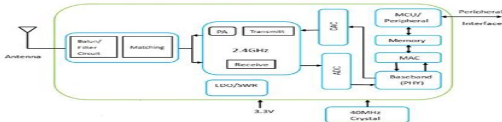
Figure 1-1 WBR3 architecture
