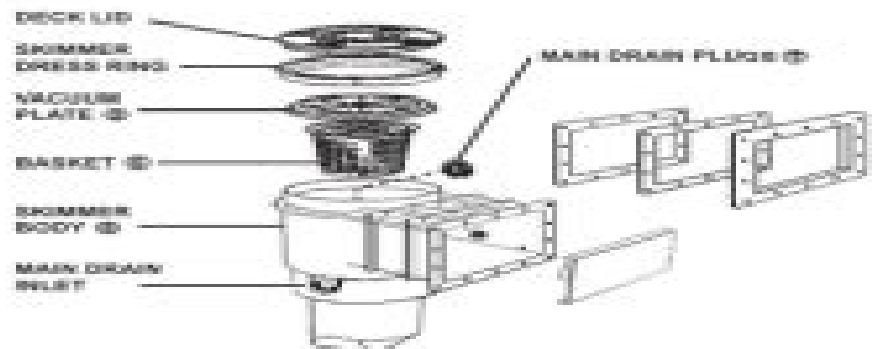
* Figure 3: S75 and Supaskimmer Skimmer Boxes
