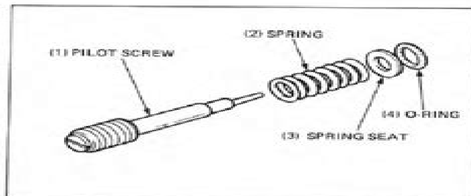
(1) PILOT SCREW
