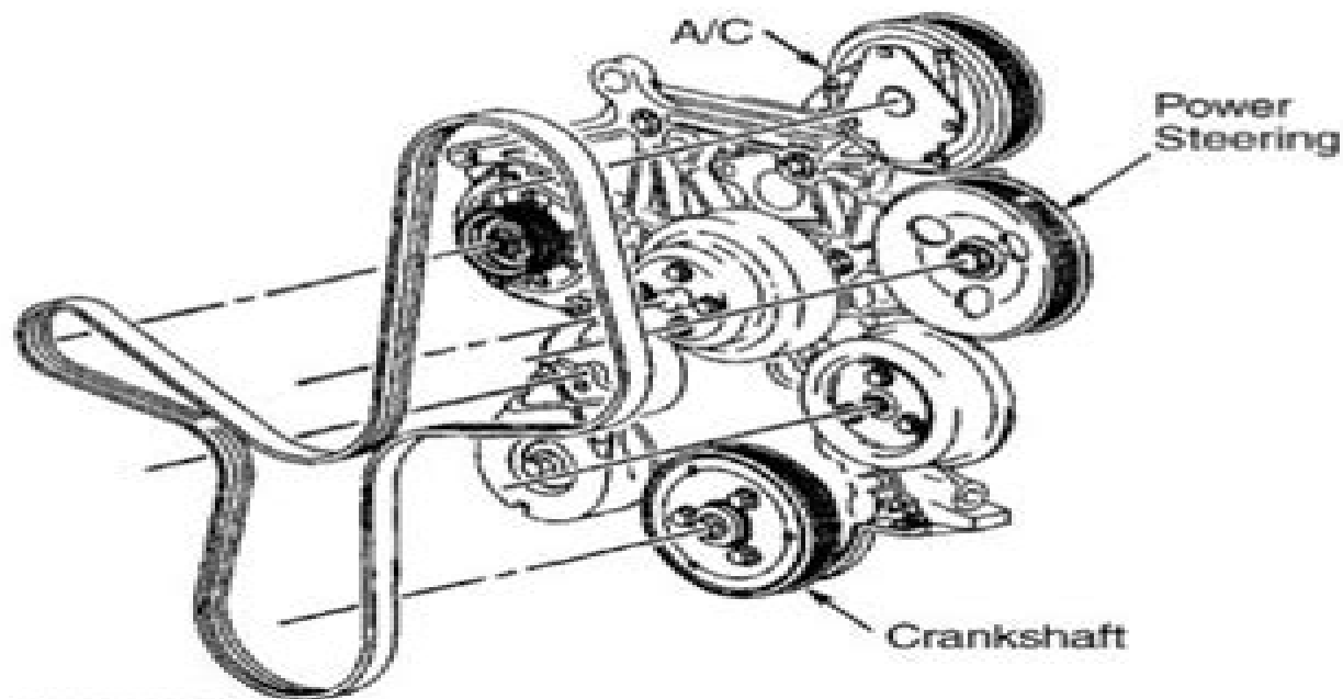
Fig. 9: Serpentine Belt Routing (2.2L "S" Pickup) Courtesy of GENERAL MOTORS CORP.
