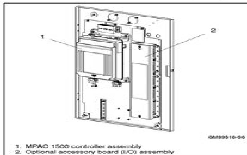
Figure 1 Decision-Maker® MPAC 1500 Controller Conversion Kit, Installed
