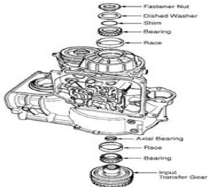
93F 10204 Fig. 47: Locating Input Transfer Gear Assembly Courtesy of Volkswagen United States, Inc.
