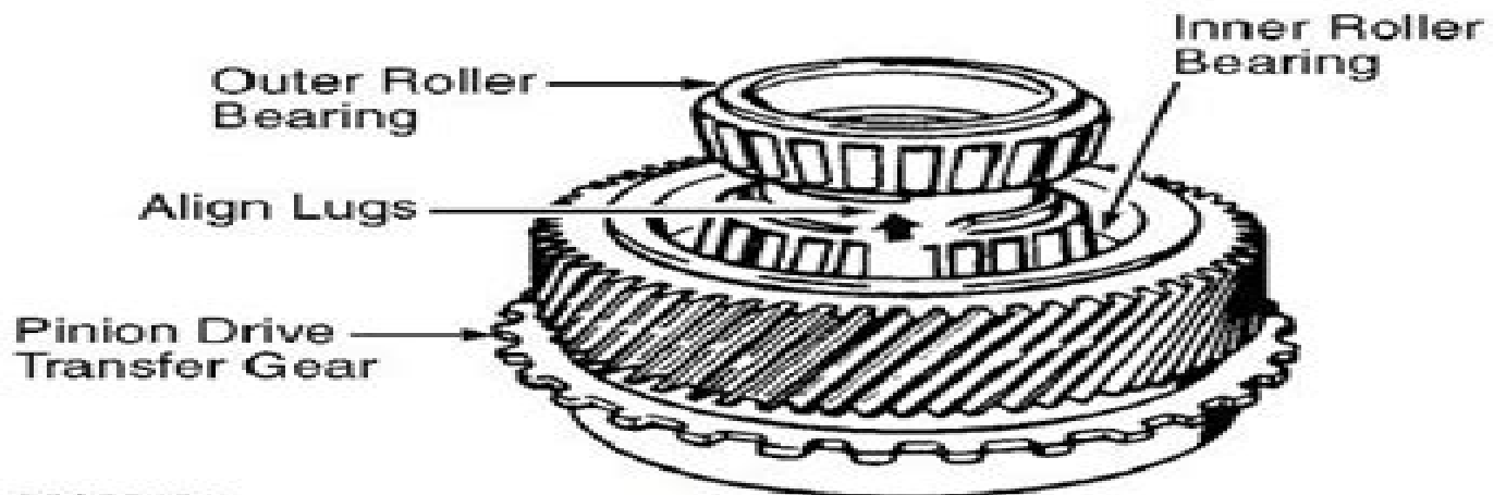
93A22491 Fig. 48: Aligning Lugs On Input Transfer Gear Roller Bearings Courtesy of Volkswagen United States, Inc.
