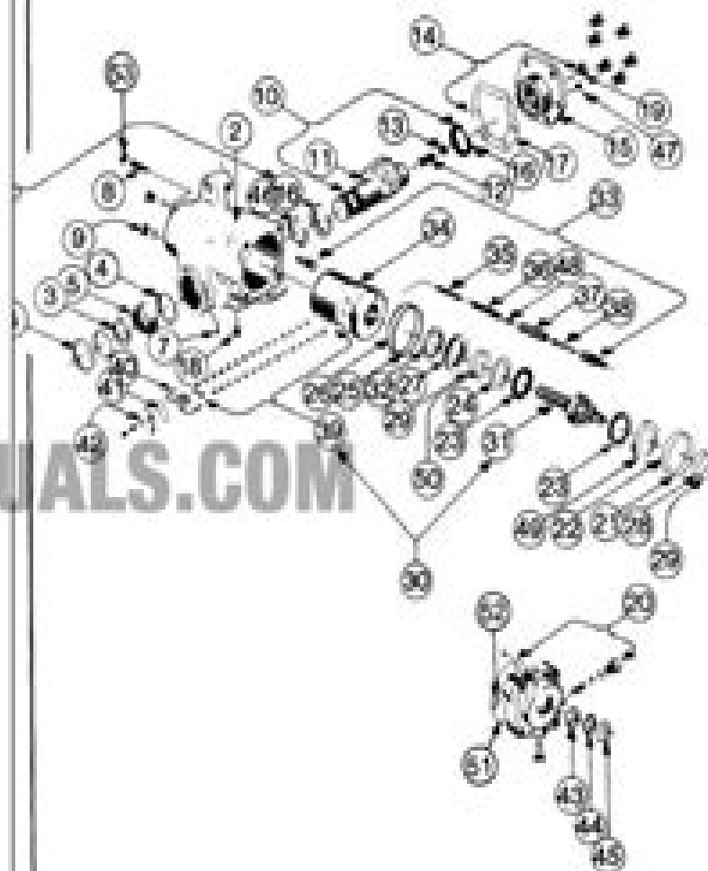
STEERING GEAR MODEL TAS-65 Fig. 30
