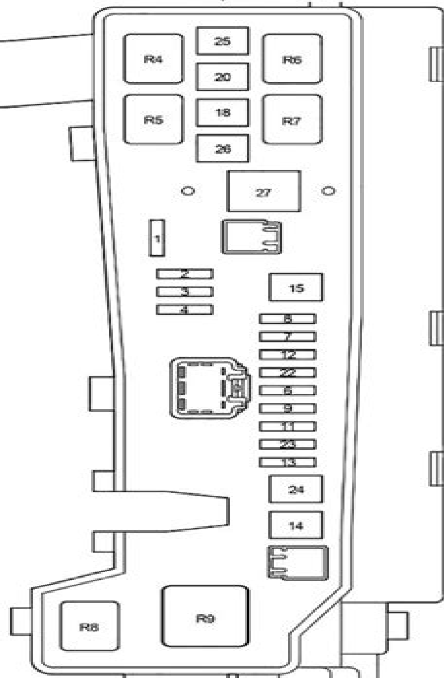
1ZZ-FE, 3ZZ-FE
