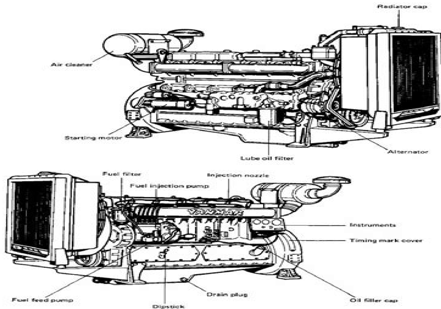
Fig. GI-2. 6HAL External view
