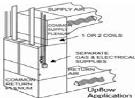
Fig 1: Up Flow Twinned Application Fig 2: Down Flow Twinned Application.
