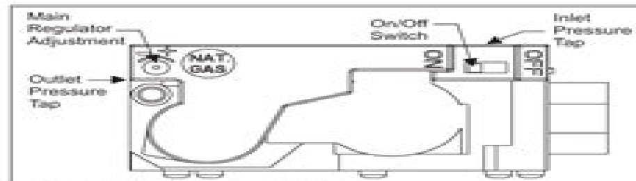
FIGURE 11: Modulating Gas Valve
