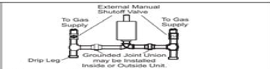
FIGURE 8: Gas Piping
