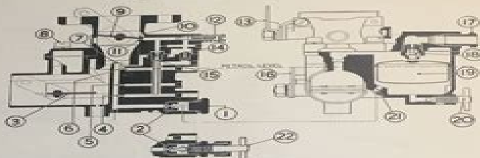
ALTERNATIVE VARIABLE MAIN JET SECTION CARBURETTOR TYPE 24T-3.
