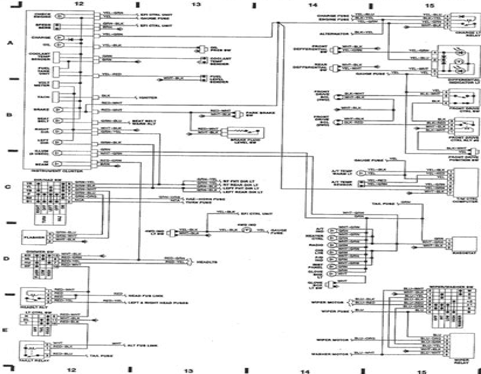
Fig. 4: Instrument Panel (Cont.) & Rear Compartment, Cluster, Hazard, Wiper/Washers 1988 Toyota Land Cruiser
