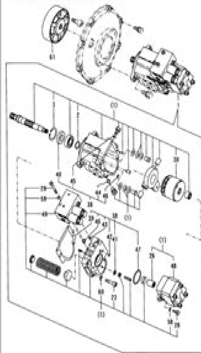
Fig. 3 HYD. OIL PUMP & JOINT
