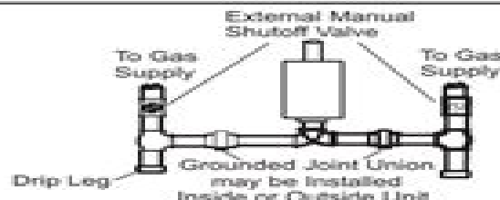
FIGURE 8: Gas Piping
