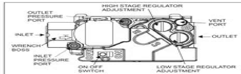
FIGURE 10: Two-Stage Gas Valve
