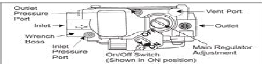
FIGURE 9: Single Stage Gas Valve
