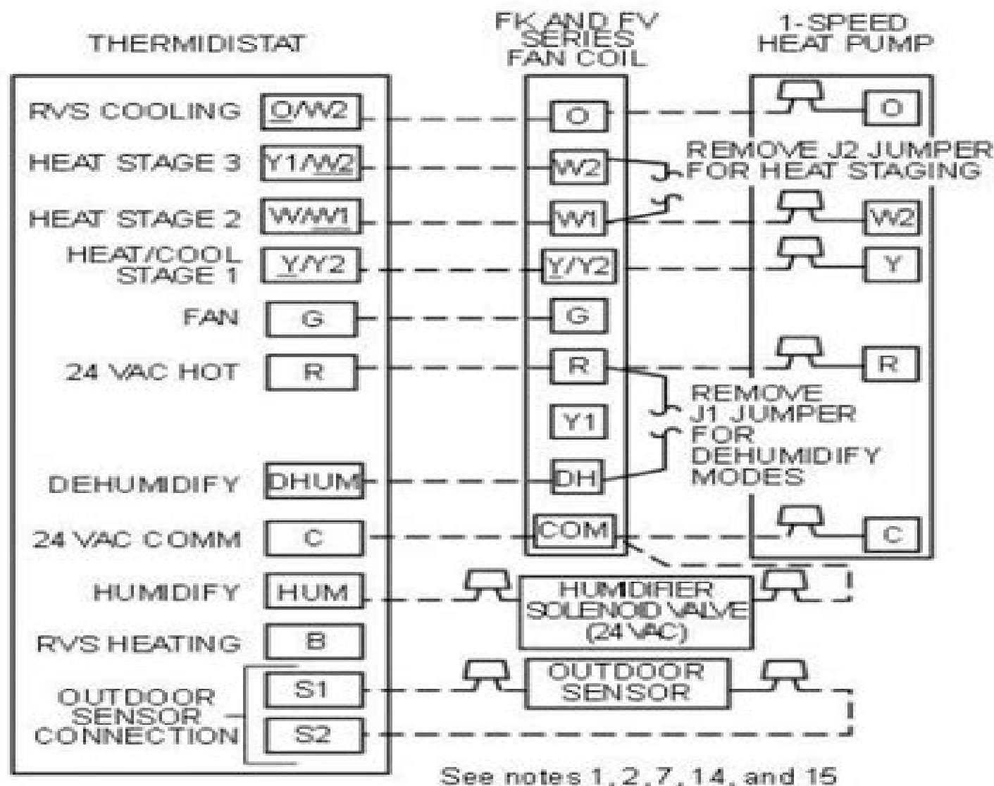
Fig. 7—FK and FV Series Fan Coil With 1-Speed Heat Pump
