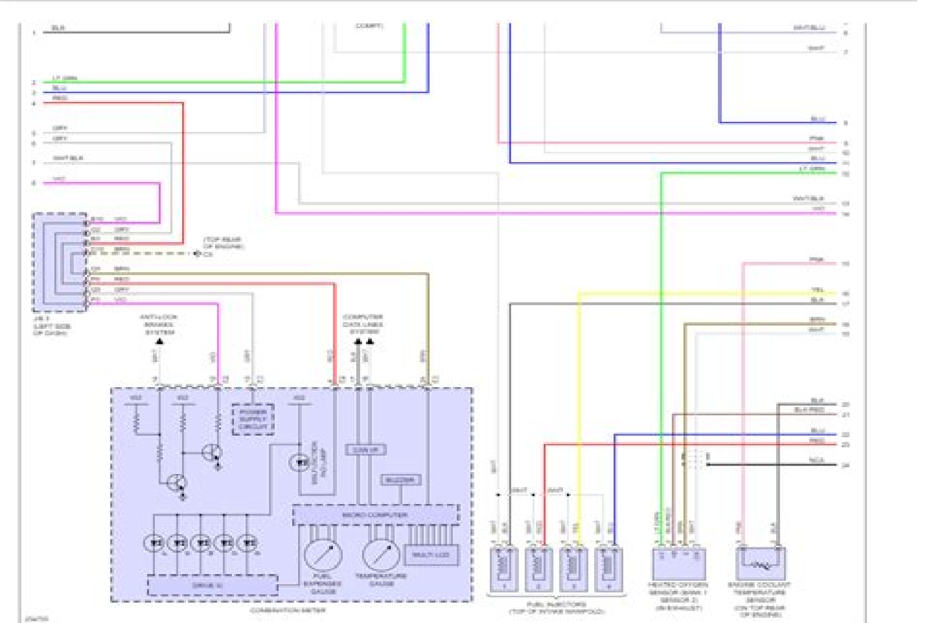
Fig 6: Hybrid System Circuit (6 of 7)
