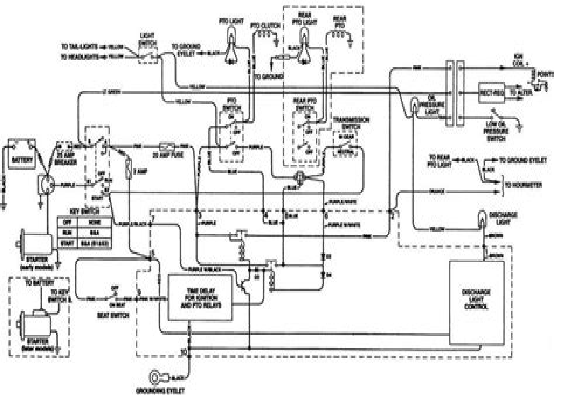
96-22-Wiring diagram for Model 316.
