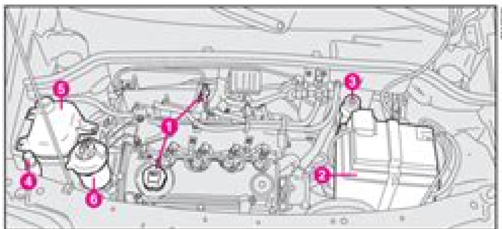
fig. 2 - 1.9 Multijet versions
