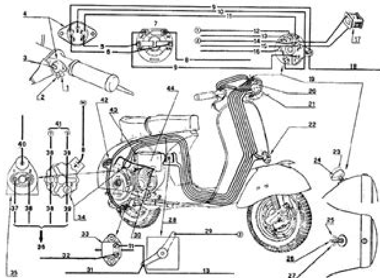
Fig. 3 - Scheme of electric wiring
