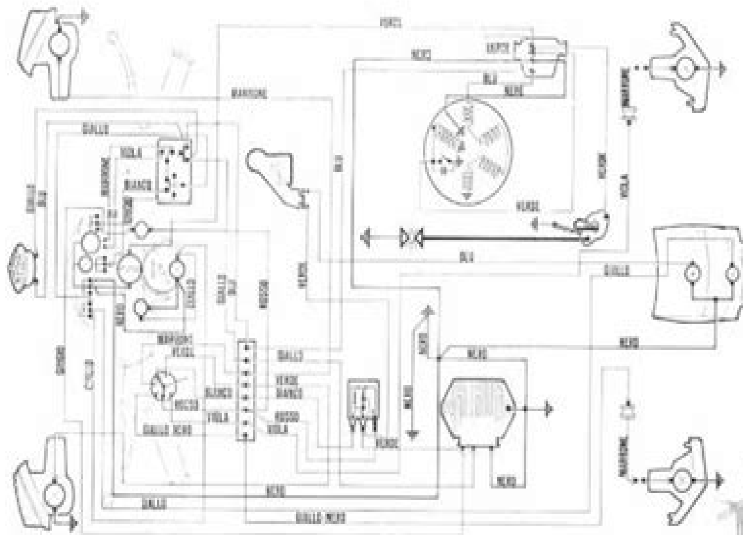
Fig. 1 - Electrical equipment diagram (P125X - P150X)
