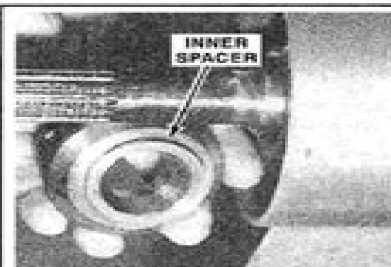
Fig. 78 For installation position the inner spacer first...
