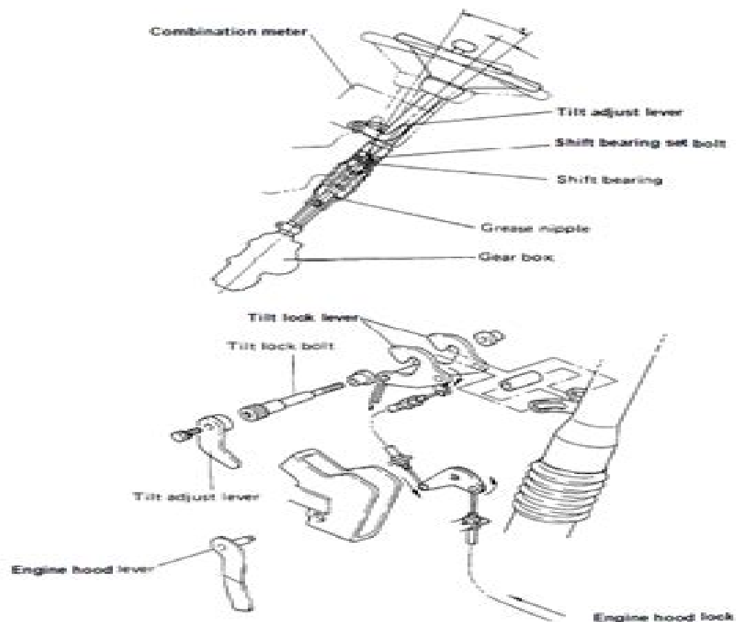
Steering Tilt System (1986.8 - 1989.8)
