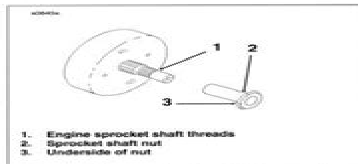
Figure 1. Compensating Sprocket Preambly
