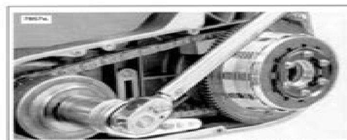
Figure 2. Tightening To 75 ft-lbs (101.7 Nm)
