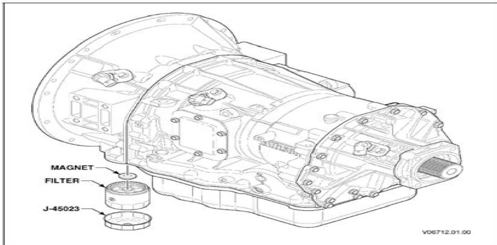
Figure 5–2. Replacing the Control Main Filter
