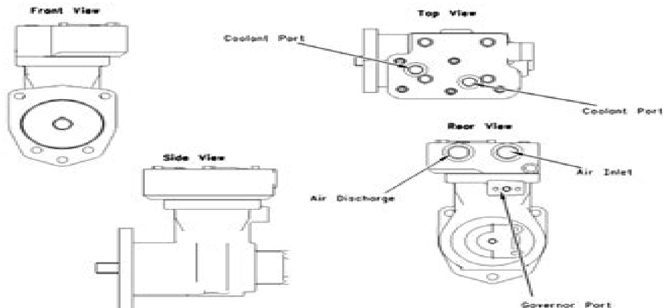
Illustration 2 Wabco 318 cc Air Compressor
