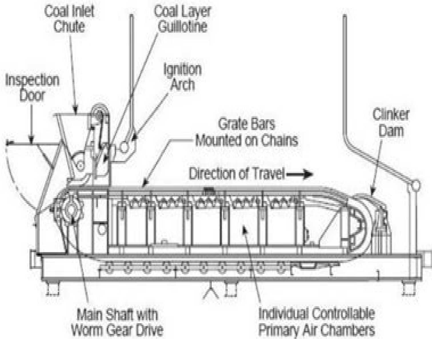
Traveling grate stoker.
