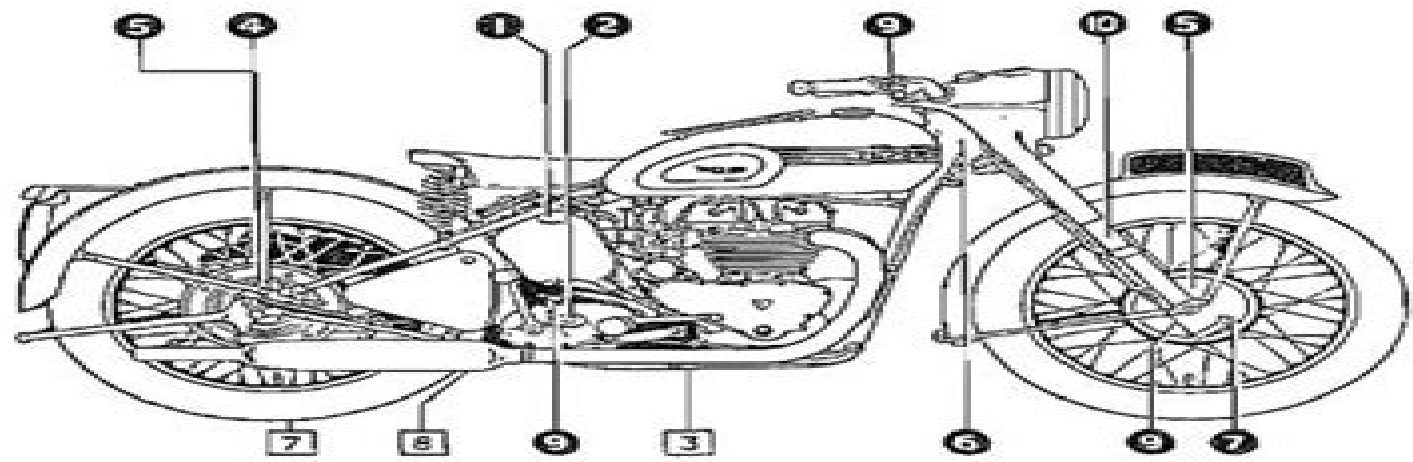
Fig. 75. LUBRICATION CHART
