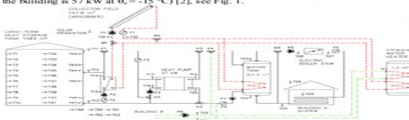
Fig. 1 – System diagram, description of key parts and measurement points of system monitoring.
