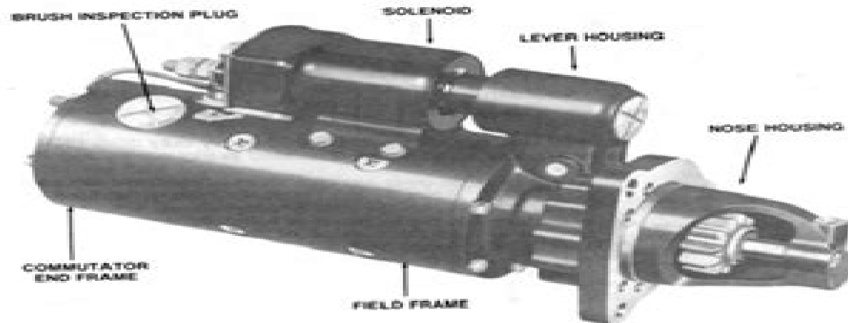
Figure 1—Typical 50-MT Series heavy duty cranking motor.
